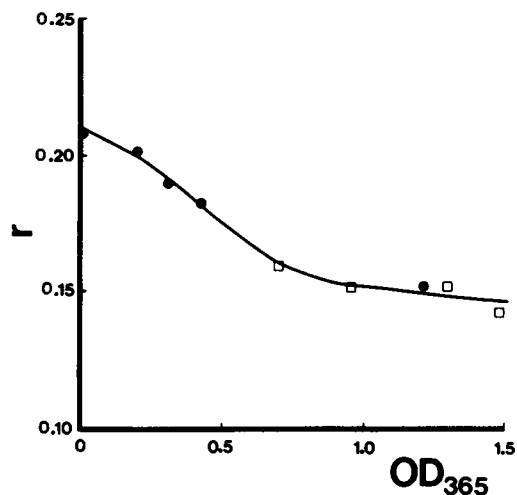
FIGURE 3 The effect of scattering on the anisotropy of DPH fluorescence for erythrocyte membrane vesicles with glass beads added to produce light scattering (●) and for intact erythrocytes (□). The optical density at 365 nm ( \text{OD}_{365} ) is used as an index of light scattering (see the text for an explanation of how this is computed for the intact erythrocytes).
